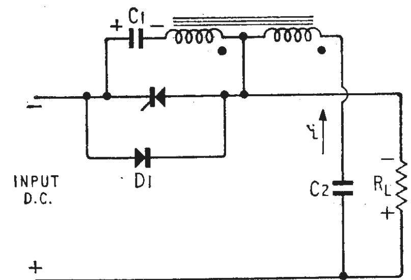
Fig. 2. Modified version of the Morgan circuit.
