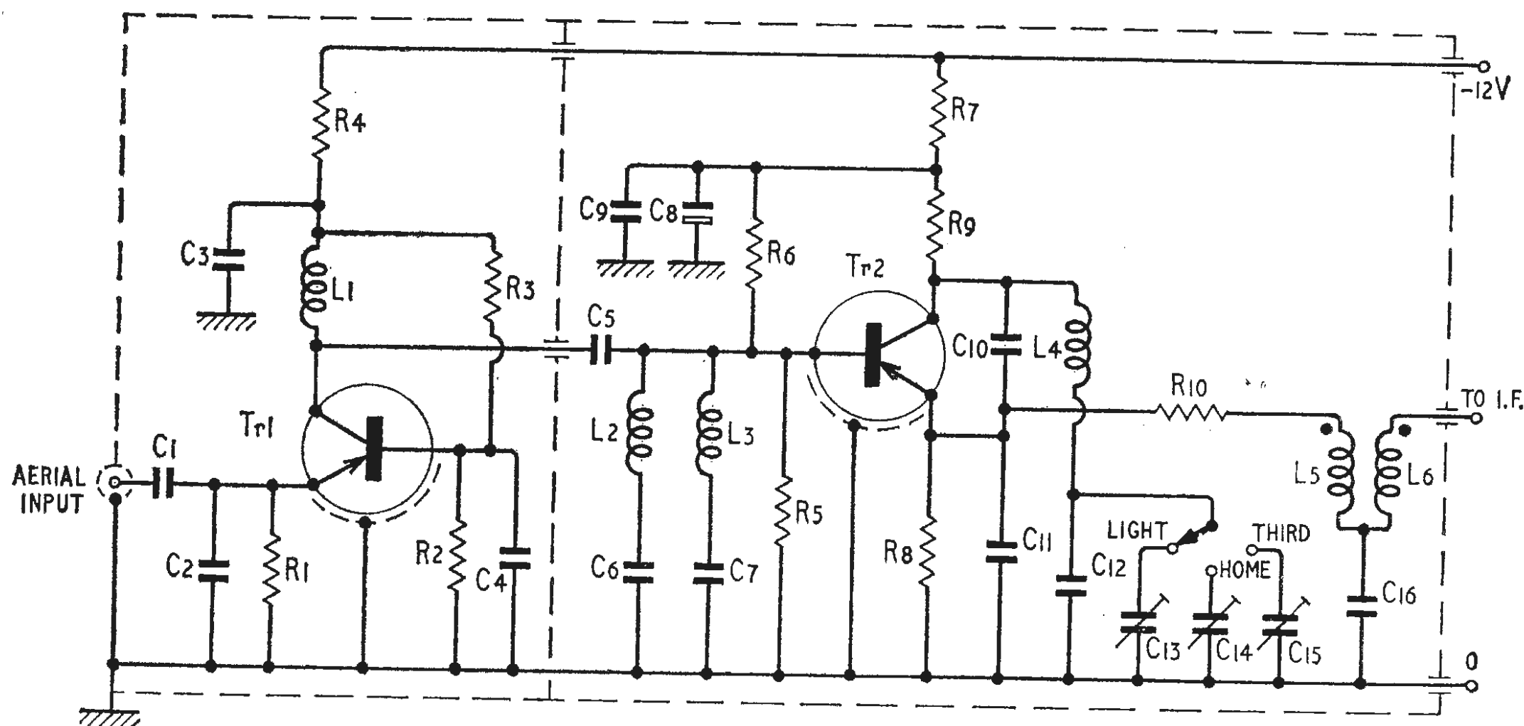
Fig. 1. R.F. and mixer stages.
