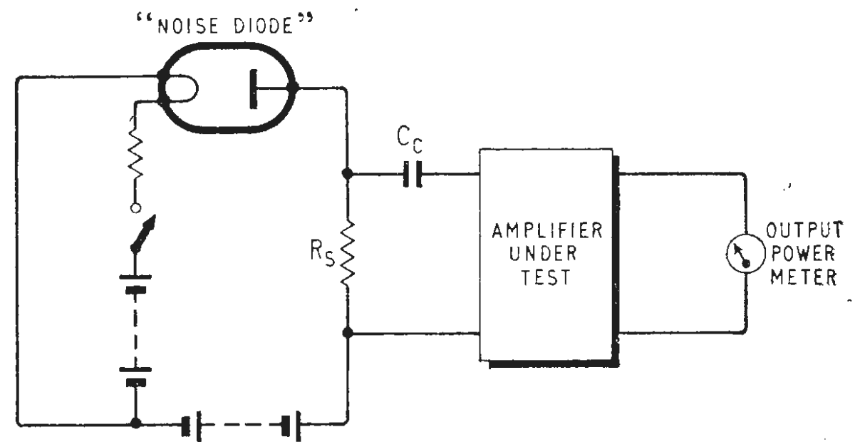
Fig. 68. Noise figure measurement circuit.
